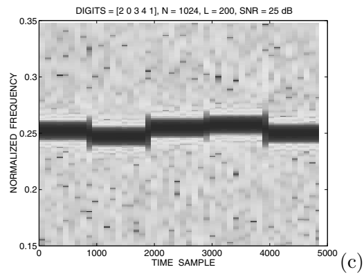
Figure 1: Frequency based coding: (a) generated IF signal, (b) frequency coded signal and (c) spectrogram of frequency coded signal.
