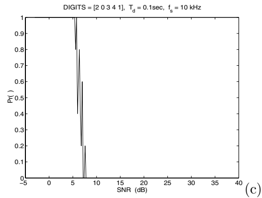
Figure 2: Frequency based decoding: (a) estimated IF signal, (b) lowpass filtered IF signal, (c) performance of decoder vs SNR.
