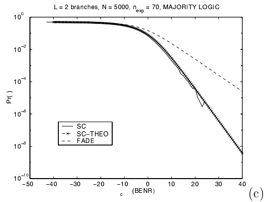
Figure 1: Binary detection in Rayleigh fading: (a) performance curves in the absence/presence of flat, Rayleigh channel fading, (b) histogram of fading activity, and (c) performance of the predetection selective combining receiver with L = 2 diversity branches.
