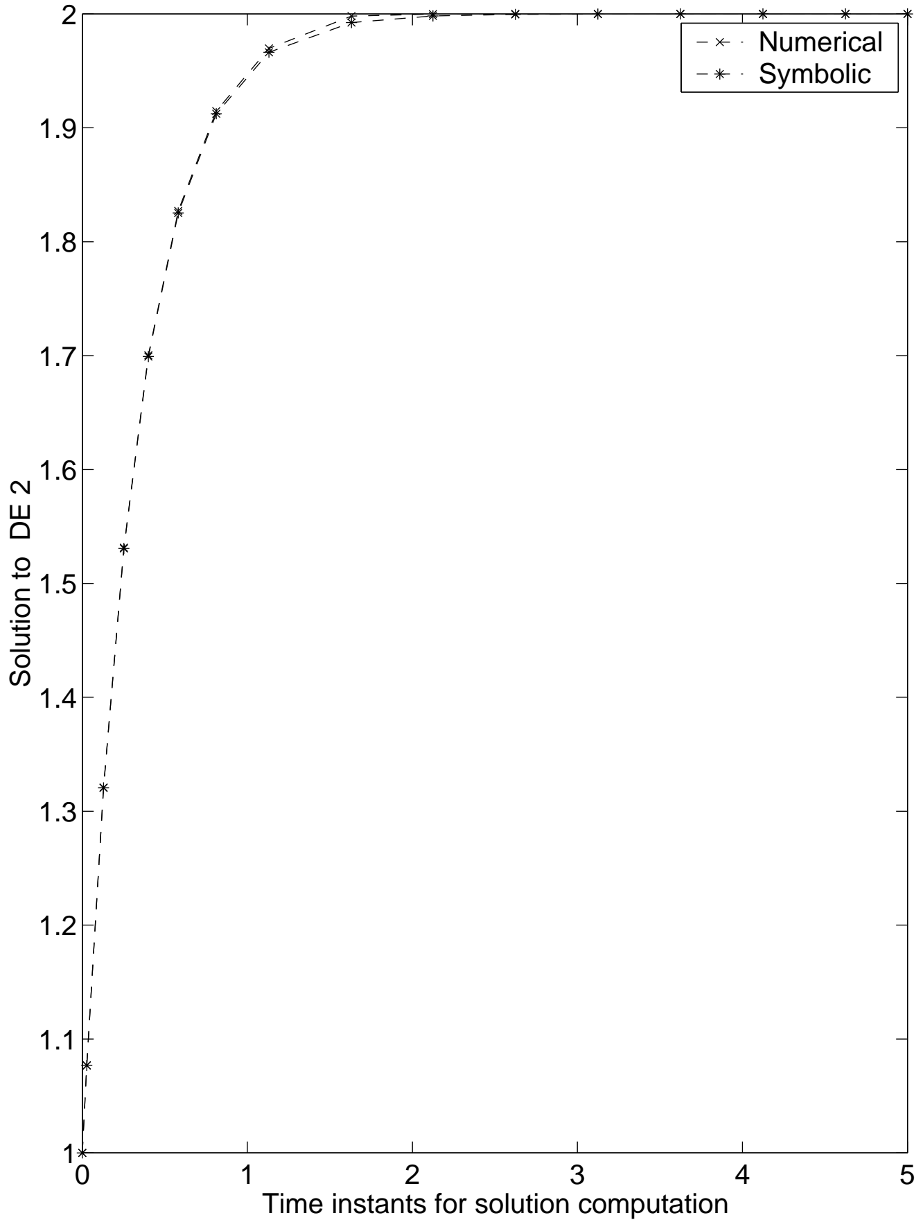
Numerical Solutions to DE via ODE solver
