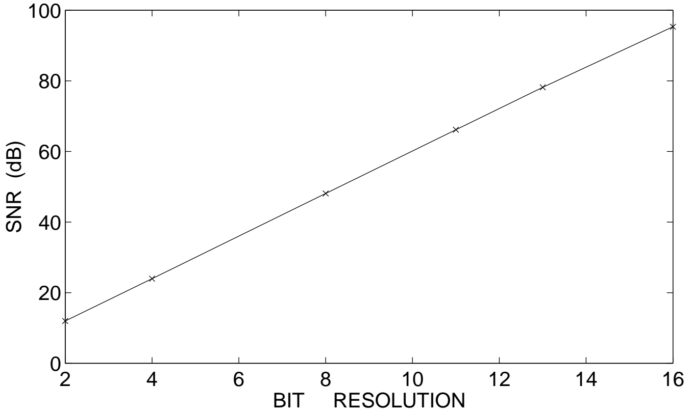
ROUND--OFF, UNIFORM QUANTIZER, SNR vs B
