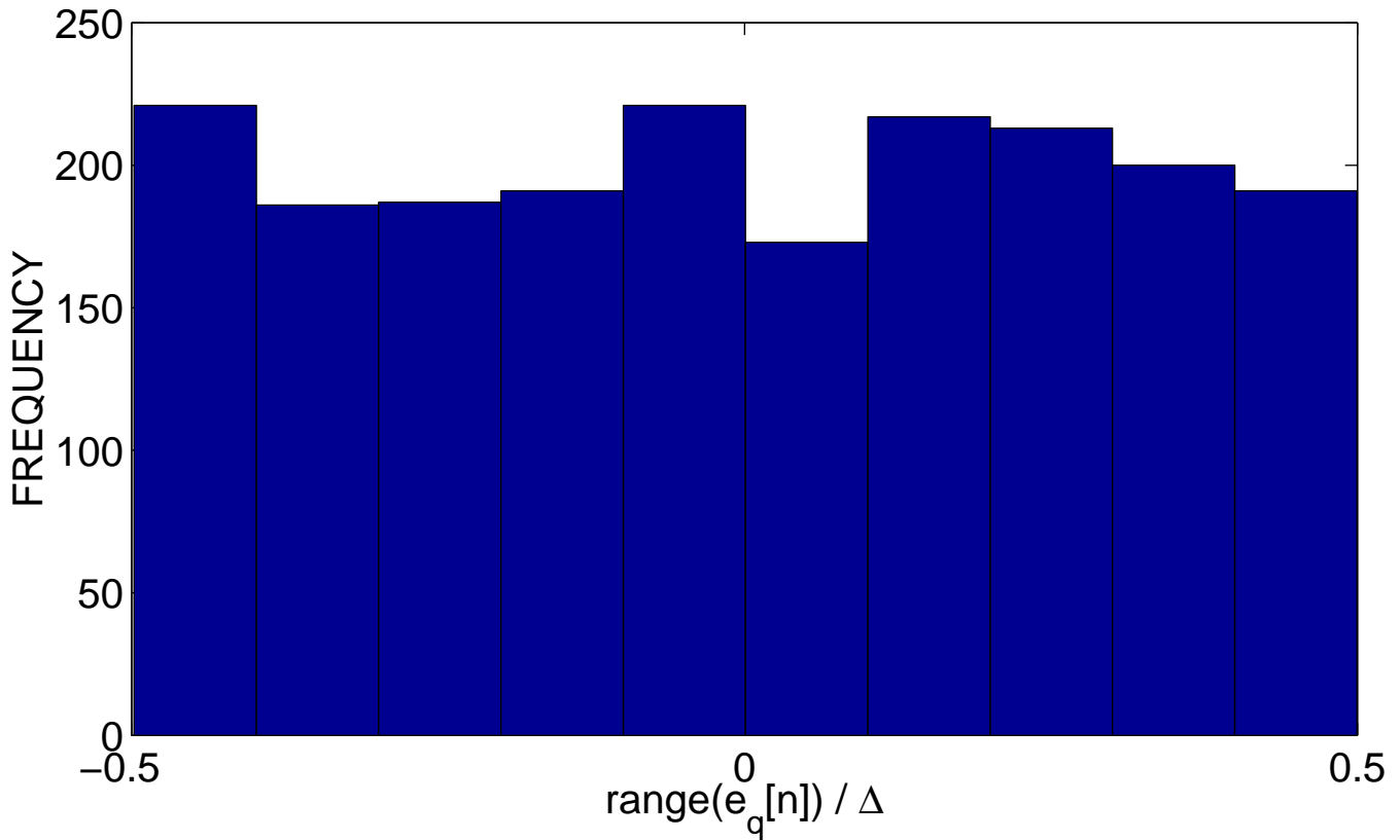
B = 12 bits, ROUND--OFF, UNIFORM SOURCE
