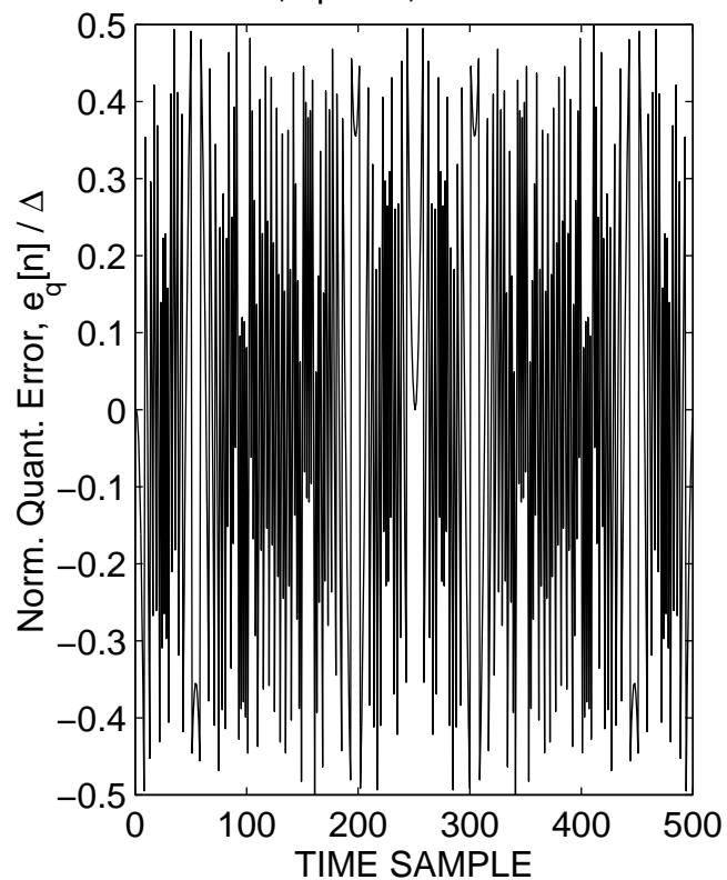
B = 7, opt = 1, SNR = 50 dB
