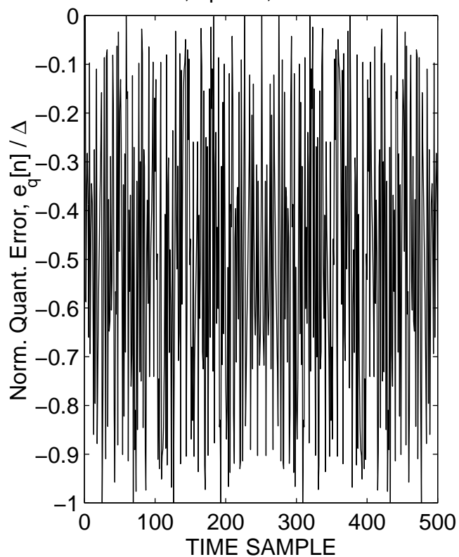
B = 15, opt = 2, SNR = 98dB
