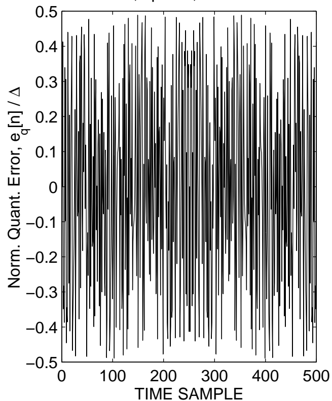
B = 15, opt = 1, SNR = 98dB
