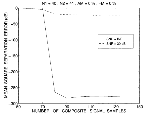
Fig. 2. Effect of AWGN on component separation in the PASSED algorithm.
