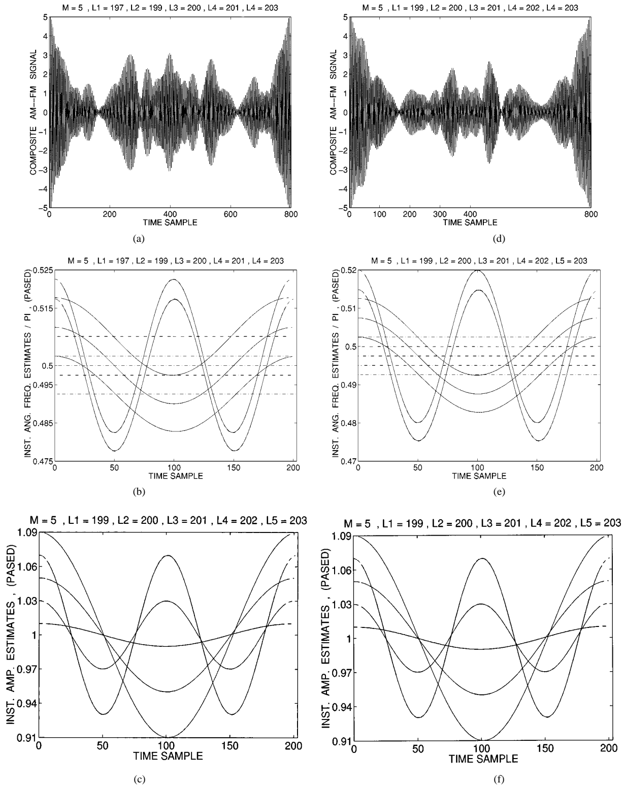
Fig. 9. Five-component example with both pairwise coprime and pairwise noncoprime component periods. (a), (d) Composite AM-FM signal. (b), (e) Angular frequency estimates of the multicomponent-PASED algorithm (as fractions of \pi ). (c), (f) IA estimates of the components via the multicomponent-PASED algorithm. Solid lines are estimates, dashed lines are actual quantities and dashed-dotted lines are carrier frequency estimates. The IF signals are sinusoidal with \{2, 4, 2, 4, 2\}\% FM. The IA signals are also sinusoidal with \kappa_i \in \{1, 3, 5, 7, 9\}\% AM.
