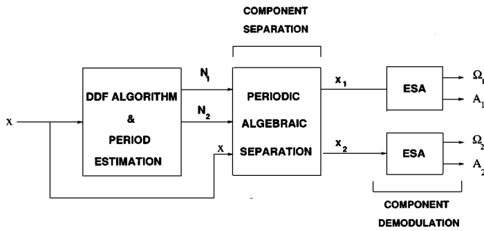
Fig. 1. Block diagram of the PASSED algorithm.
