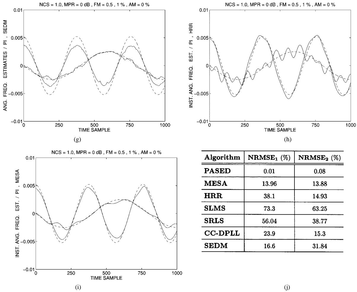
Fig. 7. (Continued.) Comparison of the PASED algorithm with other multicomponent AM-FM demodulation algorithms. (g), (h) Corresponding estimates of the SEDM and the HRR algorithms, respectively. Solid lines are the estimates and the dashed lines are the actual quantities. Post-smoothing of the IF estimates using moving average and 9-pt median filtering removes some of the interference and spikes but at the cost of distorting the IF estimates.
