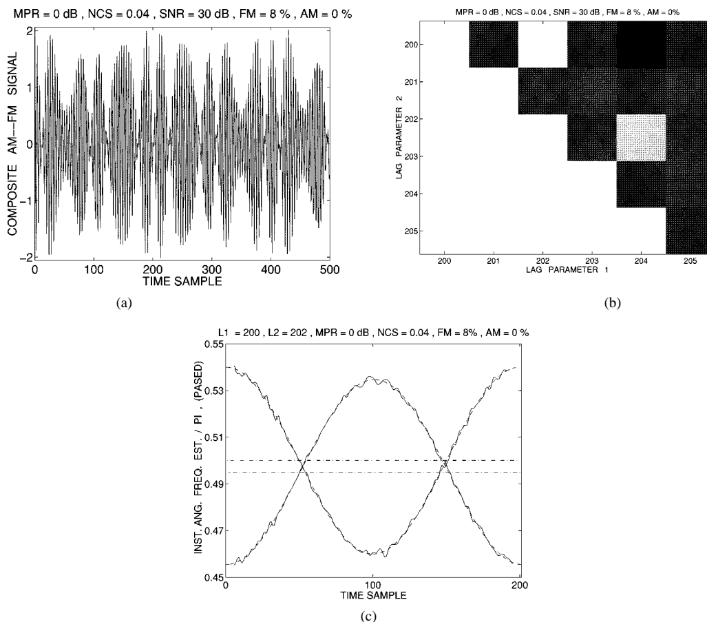
Fig. 5. Noisy AM-FM signal example with a SNR of 30 dB. Noisy example: (a) composite signal, (b) DDF over a half-quadrant search region, where dark areas indicate high DDF value and light areas indicate small DDF values, and (c) angular frequency estimates (as fractions of \pi ). The SNR of the signal mixture is 30 dB. 4-time binomial smoothing was used for smoothing the energy signals in the ESA. The IF signals are sinusoidal with 8% FM, with 4% NCS.
