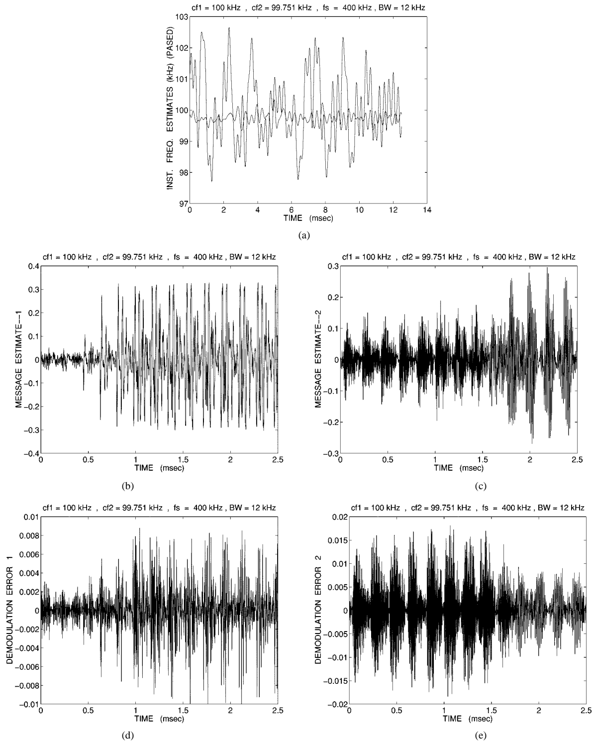
Fig. 10. PASSED-based separation and demodulation of voice-modulated cochannel FM signals. (a) Instantaneous frequency estimates of the PASSED. (b), (c) Demodulated message signals of the PASSED. (d), (e) Associated demodulation errors of the PASSED.
