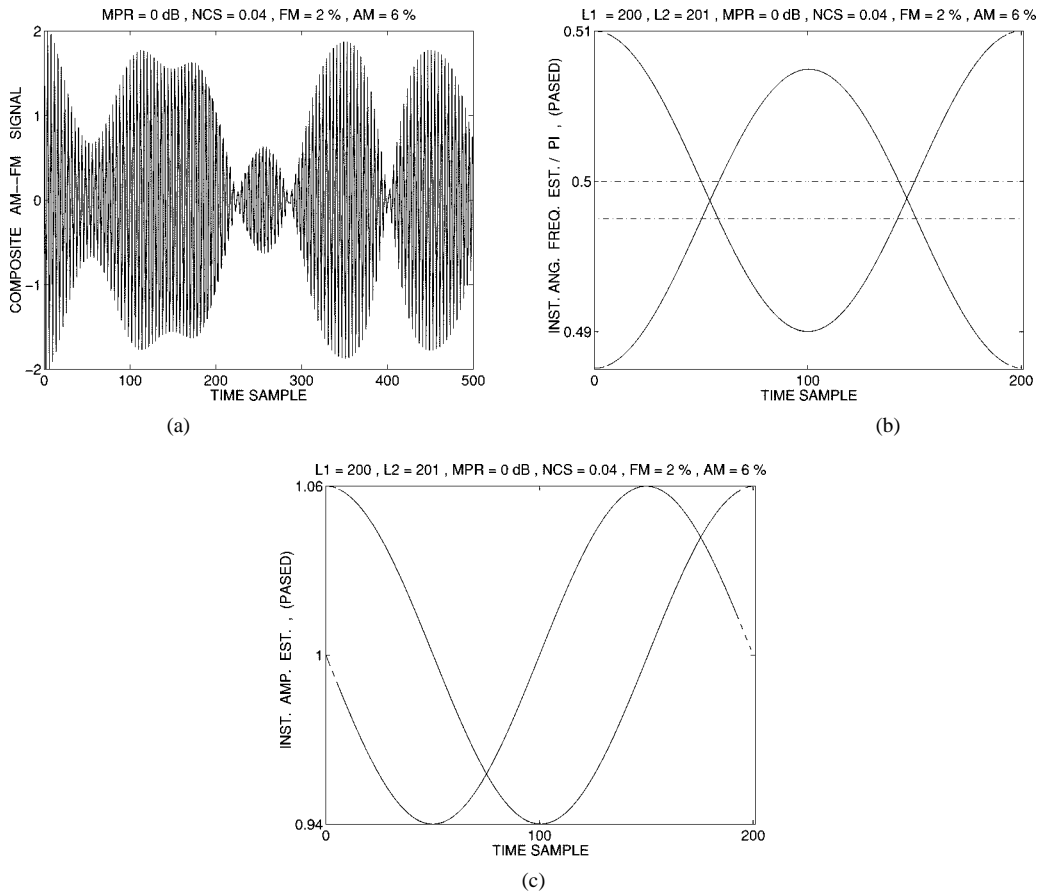
Fig. 3. Sinusoidal AM-FM example with coprime component periods. Sinusoidal AM-FM: (a) composite AM-FM signal, (b) IF and carrier estimates of the PASED algorithm (as fractions of \pi ), and (c) IA estimates of the PASED algorithm, where solid lines show estimated signals, dashed lines show original signals, and dashed-dotted lines show estimated carrier frequencies. The IF signals are sinusoidal with 2% FM, 4% NCS and coprime component periods. The IA signals are also sinusoidal with 6% AM and an MPR of 0 dB.
