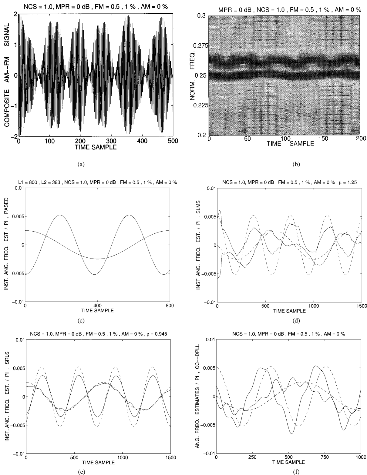
Fig. 7. Comparison of the PASSED algorithm with other multicomponent AM-FM demodulation algorithms. (a) Composite FM signal. (b) Spectrogram of the composite signal using a Hamming window of 384 samples and an FFT of 1024 samples with a time-increment of eight samples. (c) Carrier-unbiased angular IF estimates of the PASSED algorithm. (d), (e) Estimates of the SLMS and the SRLS algorithm. (f) Estimates of the CC-DPLL algorithm using a first-order loop filter. Solid lines are the estimates and the dashed lines are the actual quantities. Post-smoothing of the IF estimates using moving average and 9-pt median filtering removes some of the interference and spikes but at the cost of distorting the IF estimates.
