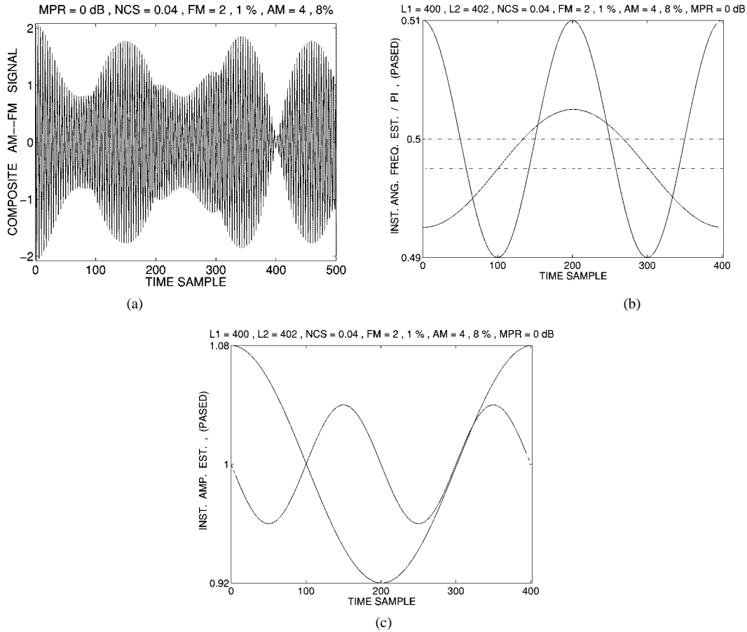
Fig. 4. Sinusoidal AM-FM example with noncoprime component periods. Noncoprime component periods: (a) composite AM-FM signal, (b) angular frequency estimates of PASSED algorithm (as fractions of \pi ), and (c) IA estimates of the PASSED algorithm, where solid lines show estimated signals, dashed lines show original signals, and dashed-dotted lines show estimated carrier frequencies. The IF signals are sinusoidal with 2, 1% FM, respectively, with 4% NCS and noncoprime component periods. The IA signals are also sinusoidal with 4, 8% AM and an MPR of 0 dB.
