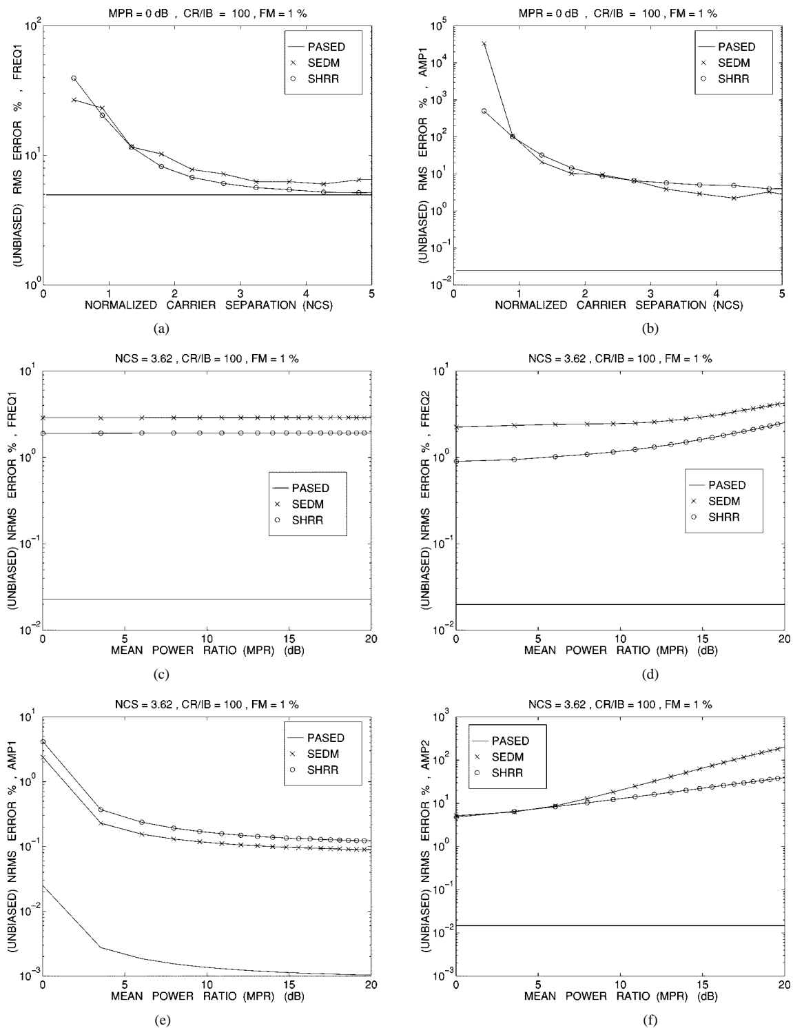
Fig. 8. Effect of NCS and MPR parameters on demodulation in the PASED, the SEDM, and the SHRR algorithms. (a), (b) Effect of NCS on frequency and amplitude demodulation in the PASED, the SEDM, and the SHRR algorithms (the other algorithms developed singularities and broke down for NCS < 0.5 ) and (c)–(f) effect of the MPR parameter on frequency and amplitude demodulation in the PASED, the SEDM, and the SHRR algorithms. Amplitude estimation in the SHRR is accomplished by integrating the IF estimates and solving a least-squares system for the amplitudes. All curves were obtained by averaging over \kappa_i \in [1 - 10]\% AM. The notation SX refers to the algorithm X with post-smoothing.
