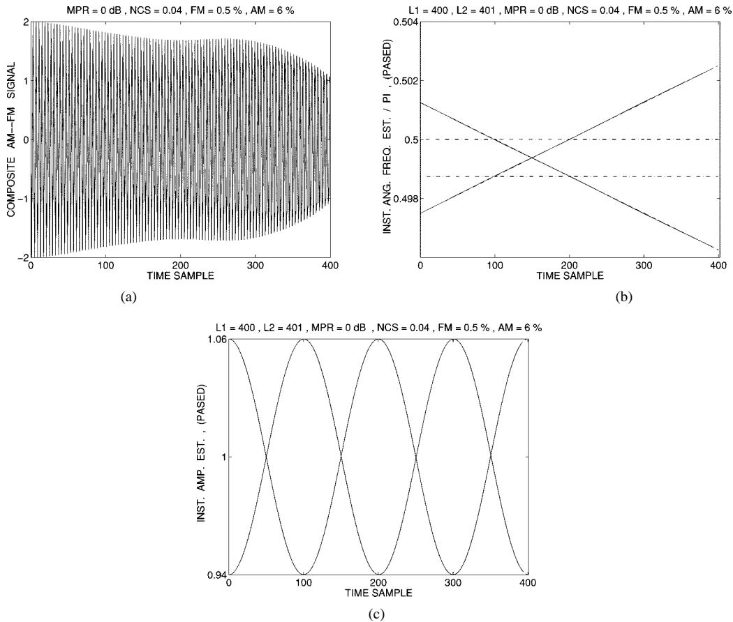
Fig. 6. Linear-FM and sinusoidal-AM example. Chirp example: (a) composite signal, (b) angular frequency estimates of the PASED algorithm (as fractions of \pi ), and (c) IA estimates of the PASED algorithm. Solid lines here indicate estimates, dashed lines indicate actual quantities and dashed-dotted lines are carrier frequency estimates. The component IF signals are linear with 0.5% FM and mutually coprime component periods with a NCS of \approx 4\% , while the IA signals are sinusoidal with an MPR parameter of 0 dB and 6% AM.
