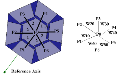
Fig.2 Antenna Structure in [3] and its graph model for all possible connections
