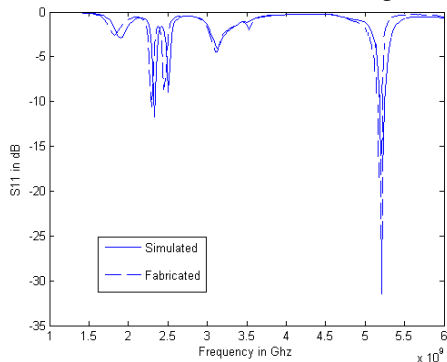
Fig.9. A comparison between the simulated and tested S11 results for the optimal antenna
