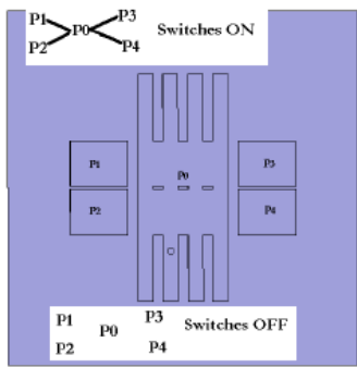
Fig.6. The optimal structure and its graph model
