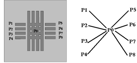
Fig.4. Antenna Structure in [6] and its graph model
