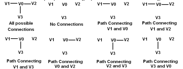
Fig.3. An example of all possible unique paths in a given graph
