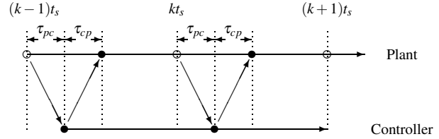
Fig. 5. Time-delay between plant and controller.
