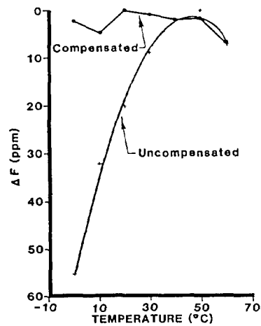
TCSO FREQUENCY vs. TEMPERATURE
