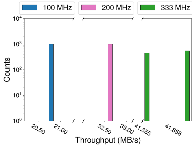
FIGURE 10: Throughput histogram for AXI-Lite GPIO for the 'Through LPD' configuration (companion graph to Fig. 9).
