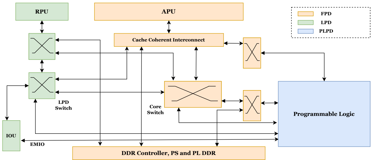
FIGURE 3: Zynq MPSoC system architecture showing microprocessors, programmable logic, DDR and interconnect.
