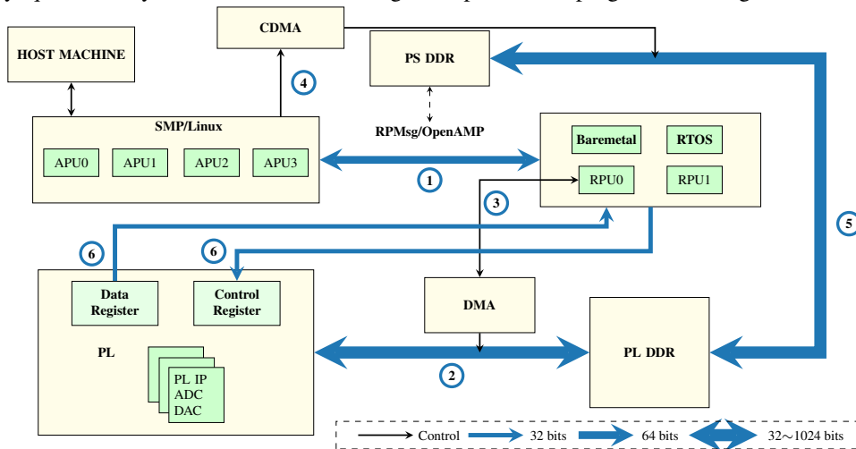
FIGURE 4: Zynq MPSoC communication channels.
