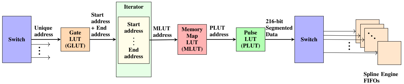
FIGURE 2: LUT architecture utilized for representing compressed gate sequences. A more detailed description of how gate sequences are generated is provided in the appendix (VIII-B).
