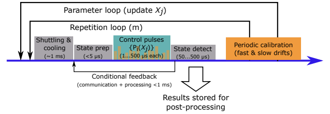
FIGURE 1: A typical experimental cycle for a trapped-ion quantum computer. A gate sequence consisting of preparation, a series of n control pulses (where i \in \{1, n\} ), and measurement/state detection, which is repeated m times for statistics. There are o different parameters that define these individual pulses (where j \in \{1, o\} ), which are updated in the parameter loop. Periodic calibration occurs on fast and slow time scales to correct for drift and other hardware errors. The electronics described here are also capable of conditional feedback such that pulse parameters can be modified based on individual or groups of measurements. More commonly the results are stored for post-processing.
