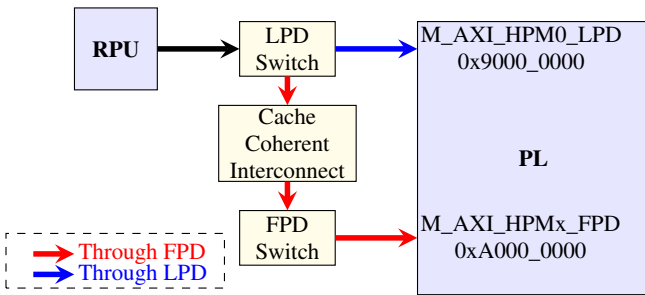
FIGURE 6: Routing network for two AXI-Lite GPIO configurations.
