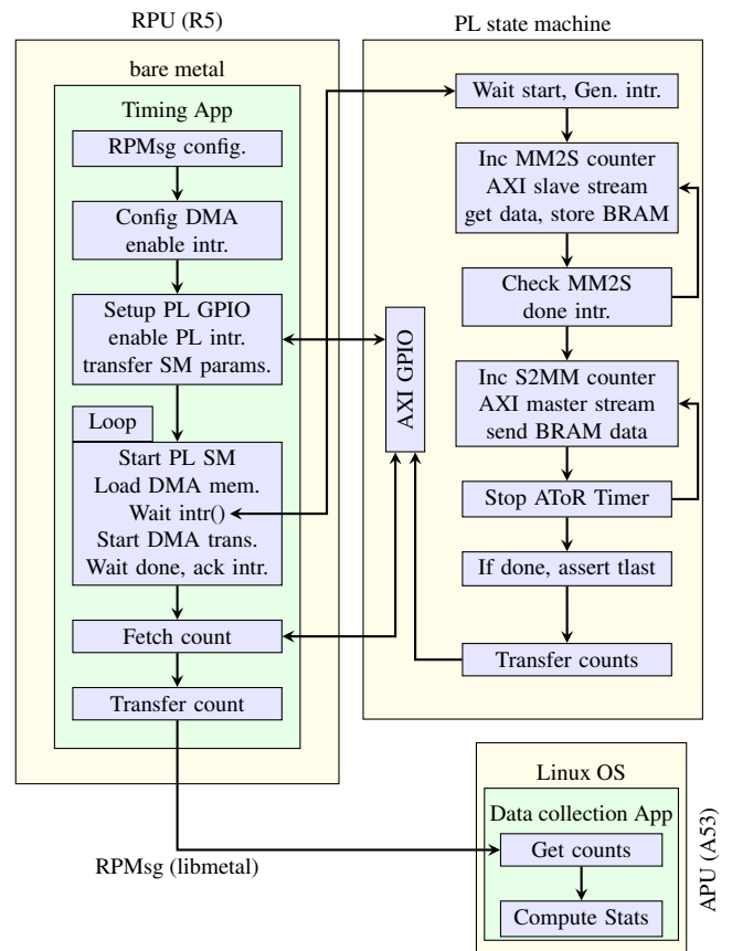
FIGURE 15: Flow diagram for DMA transfers between the RPU and an AXIS interface implemented in a PL state machine. The RPU is configured to use PL DDR for the data transfers.
