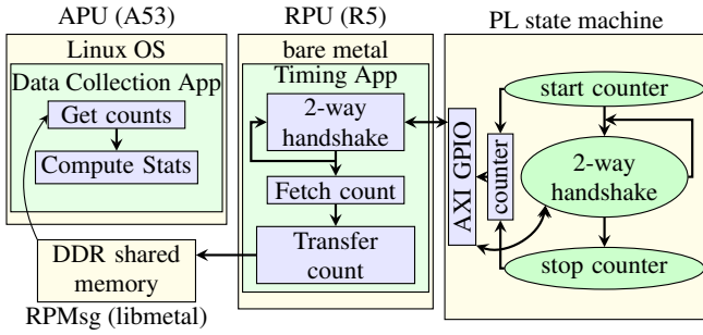
FIGURE 5: Block diagram showing architecture for timing measurements between the APU, RPU and programmable logic.
