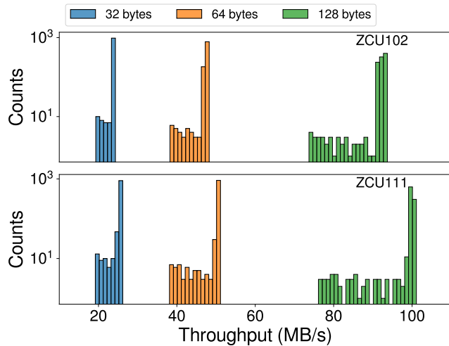
FIGURE 16: DMA MM2S throughput for the ZCU111 PL running at 333 MHz and the ZCU102 PL running at 300 MHz for payload sizes of 32, 64 and 128 B, and with the DMA data-bus bit-width set to 256.
