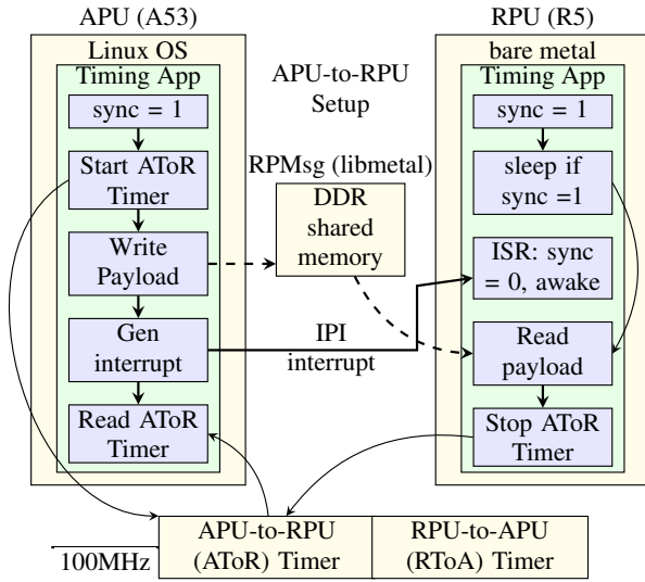
FIGURE 11: Flow diagram of RPMsg experiment for timing data transfers from APU to RPU. The sequence of operations for measuring throughput from the RPU to APU are identical but reversed.
