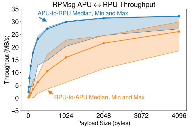
FIGURE 14: RPMsg throughput on the ZCU111 showing the median, min, and max throughput characteristics using measurements from 100,000 trials for transfers in both directions, i.e. from APU to RPU (blue) and from RPU to APU (brown).
