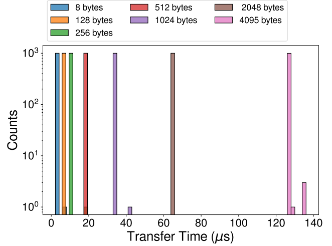
FIGURE 13: Histogram depicting RPMsg transfer times in microseconds for transfers from the RPU to the APU on the ZCU111.
