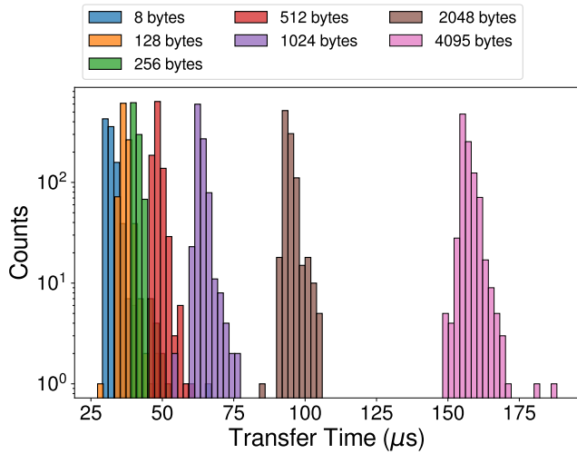
FIGURE 12: Histogram depicting RPMsg transfer times in microseconds for transfers from the APU to the RPU on the ZCU111. The y data is plotted on a \log_{10} -based scale to better emphasize variability in the measurements.
