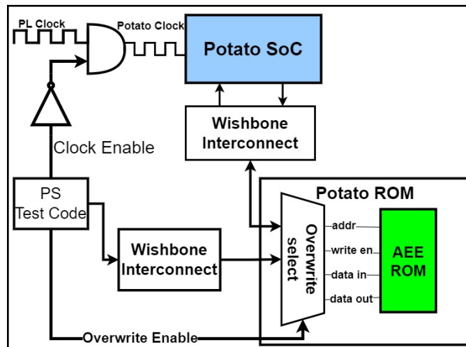
Figure 4. Block diagram of the Wishbone Side-Load architecture.
