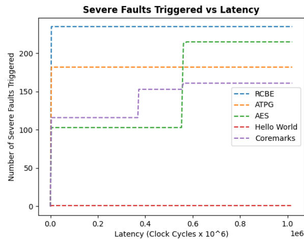
Figure 10. Subset of fault trigger latencies for select binaries
