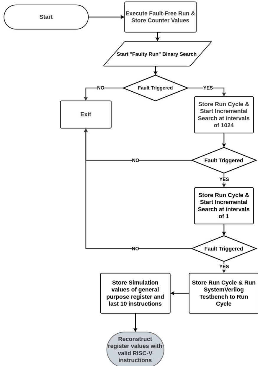
Figure 5. Flowchart for generating the RCBE
