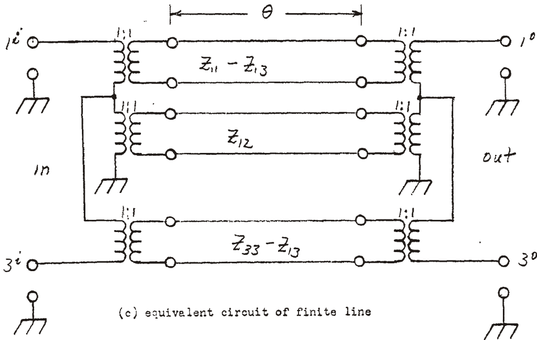
Fig.5. Equivalent circuit of a 2-line.
