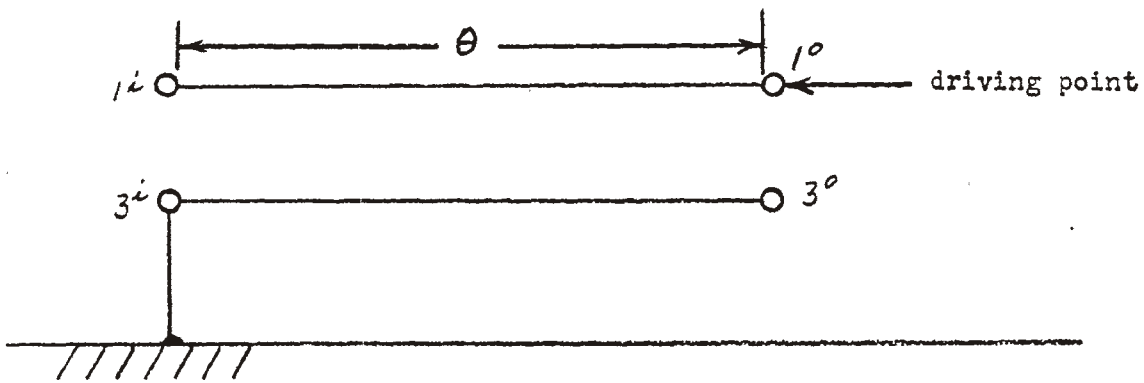
Fig.7. Schematic for determination of output admittance
