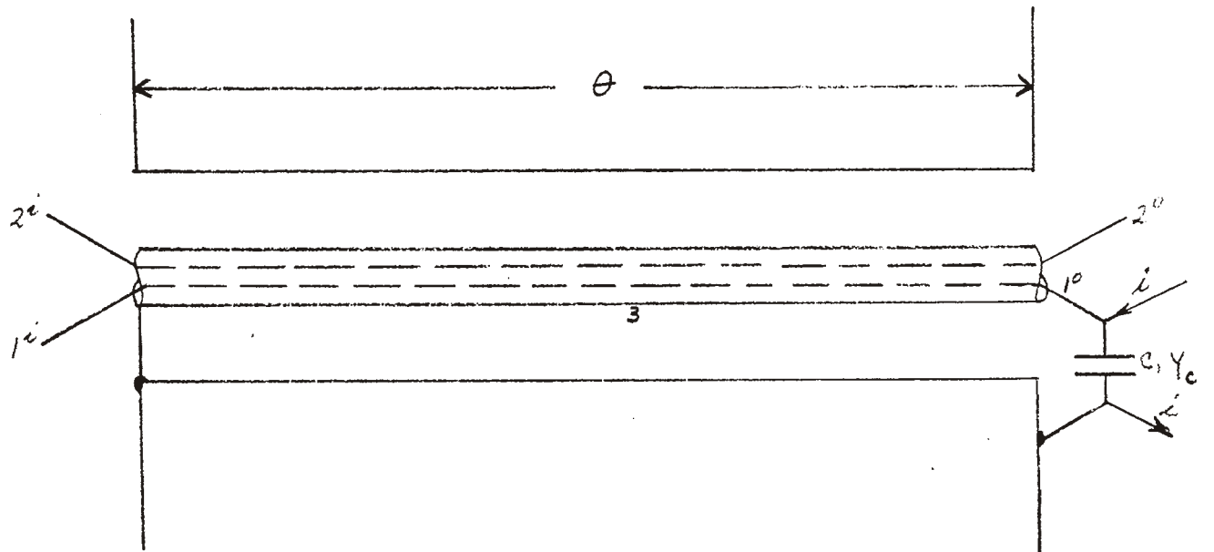
Fig.4. Compensation theorem applied to shielded pair with unbalanced load.
