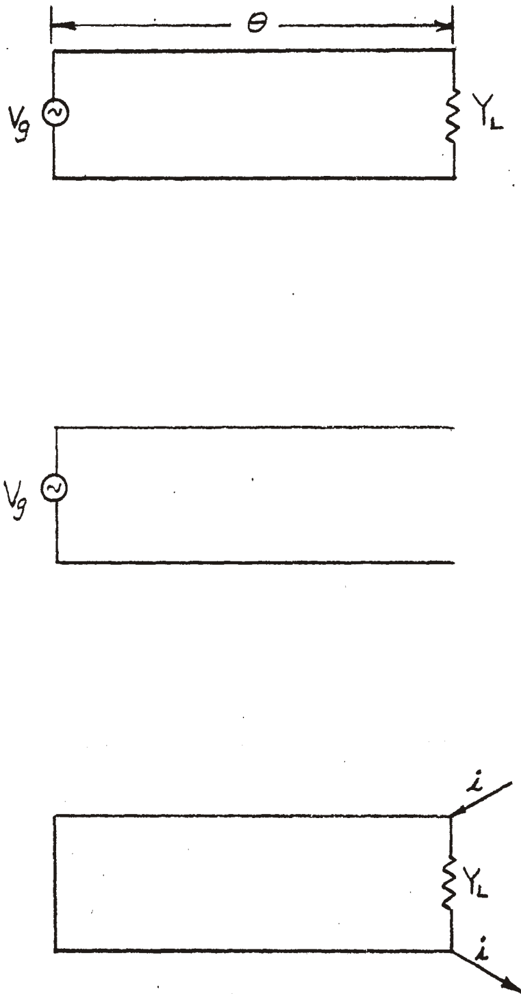
Fig.1. Current-compensation theorem illustrated.
