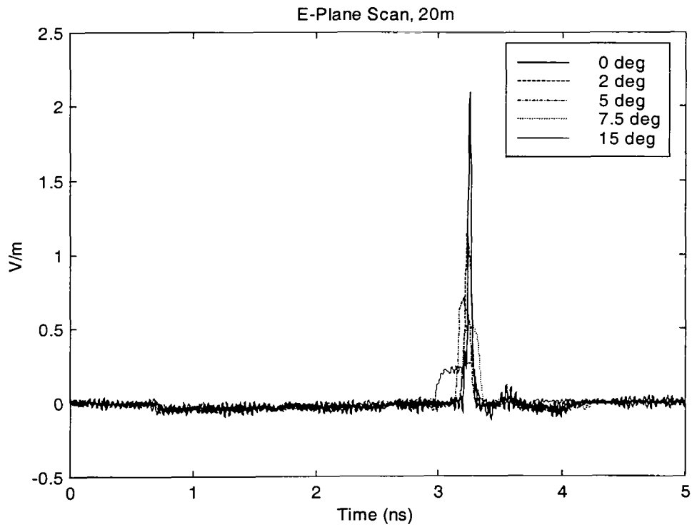
Figure 2.23. E Plane Scan at 20 m.
