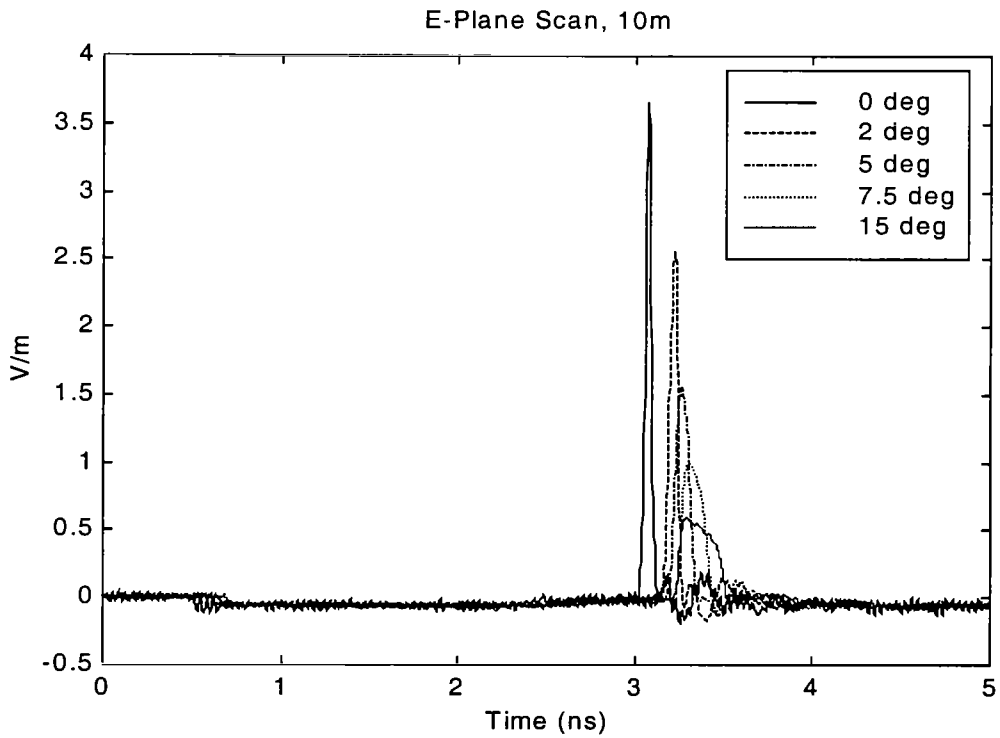
Figure 2.14. E Plane Scan (downward) at 10 m.
