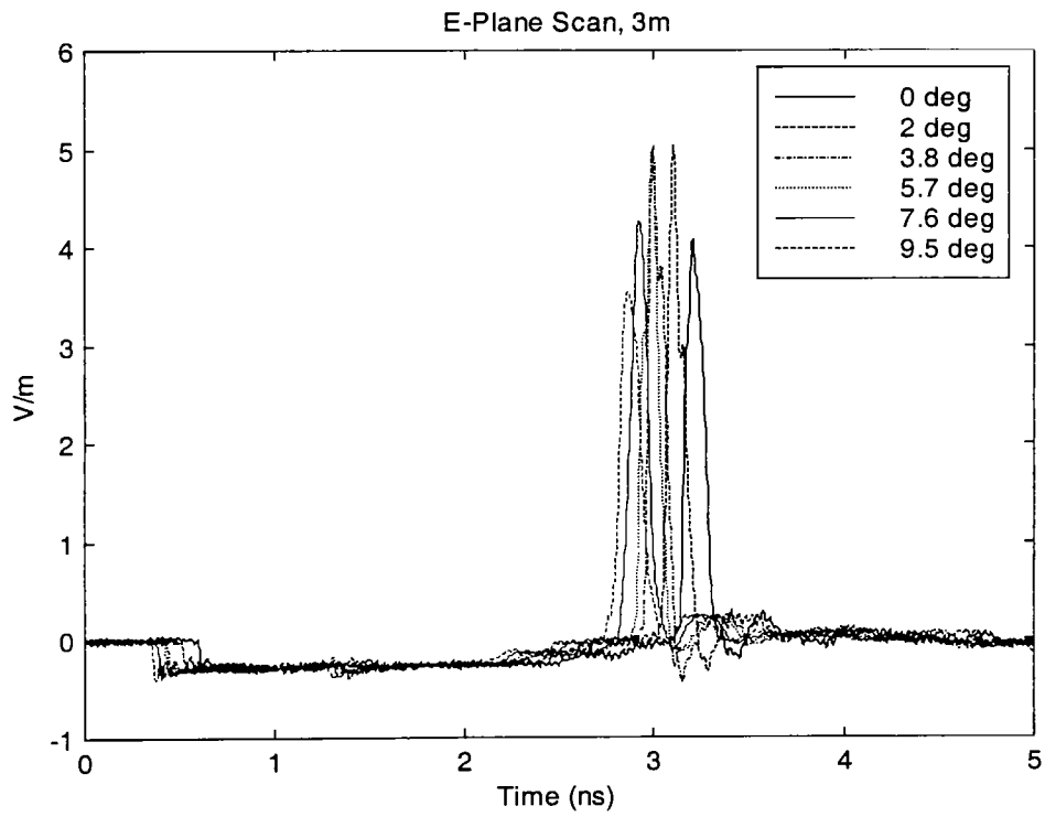
Figure 2.8. E Plane Scan at 3 m.
