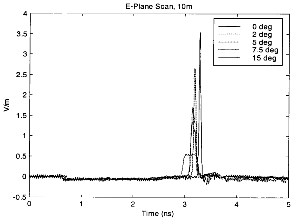
Figure 2.13. E Plane Scan (skyward) at 10 m.
