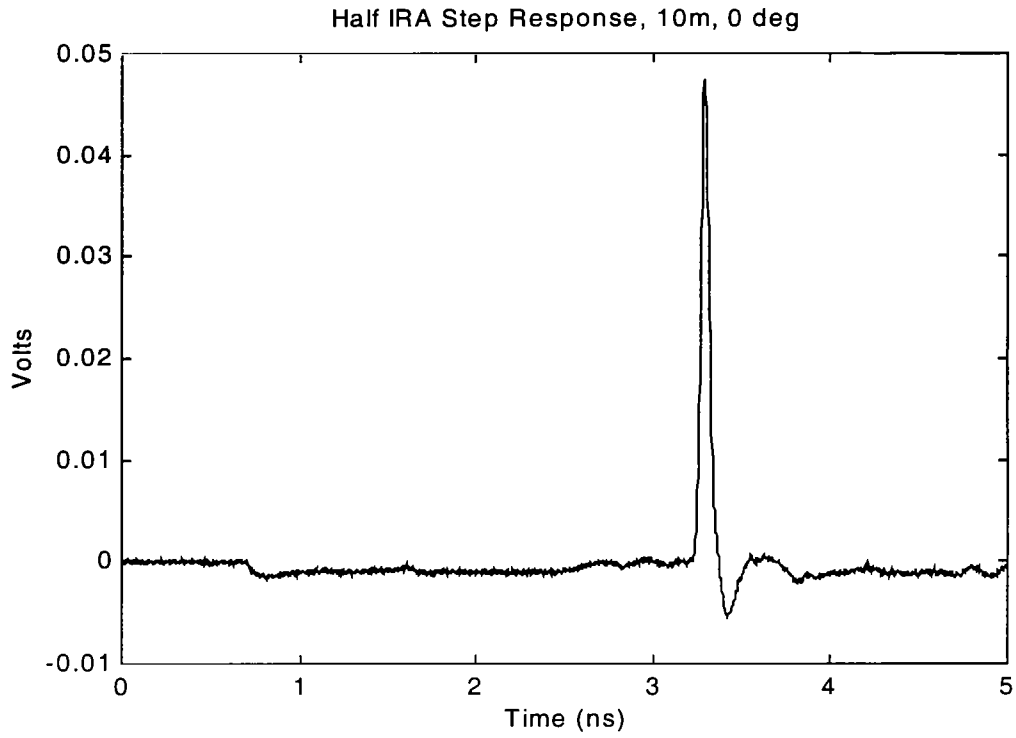
Figure 2.9. Measured Voltage on Boresight at 10 m.
