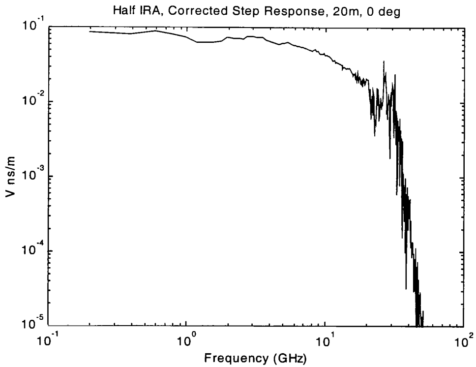
Figure 2.21. HIRA Corrected Step Response on Boresight at 20 m.
