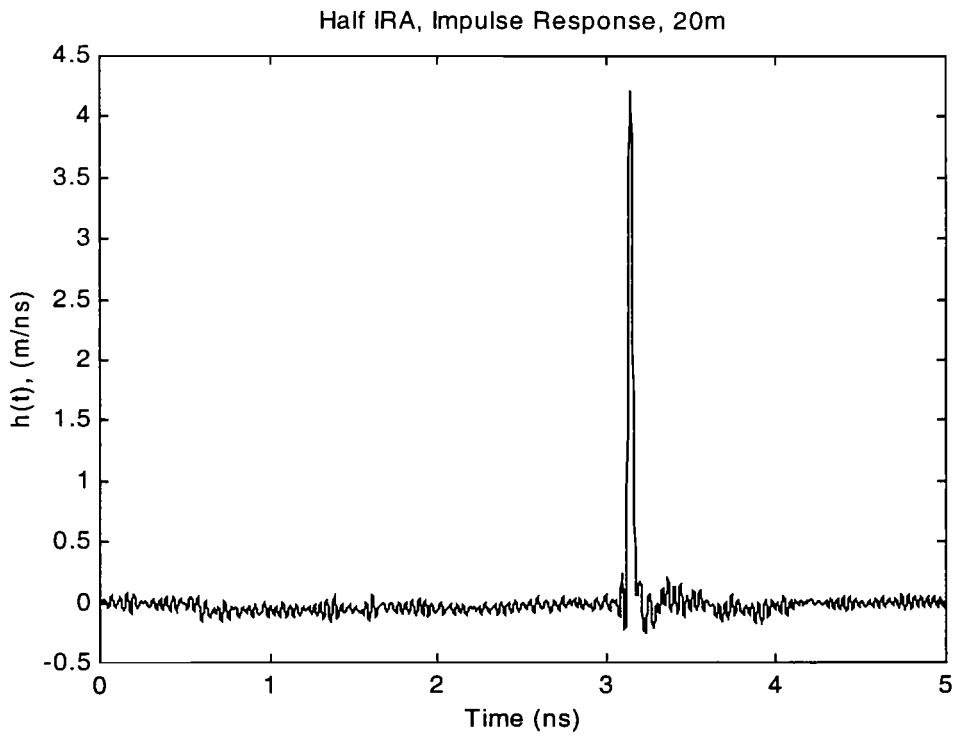
Figure 2.2 HIRA Impulse Response ( h_{HIRA}(t) ) on Boresight.
