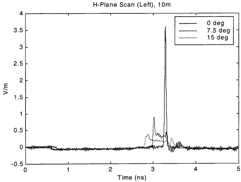
Figure 2.12. H Plane Scan (to left) at 10 m.
