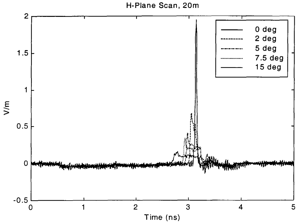
Figure 2.22. H Plane Scan at 20 m.
