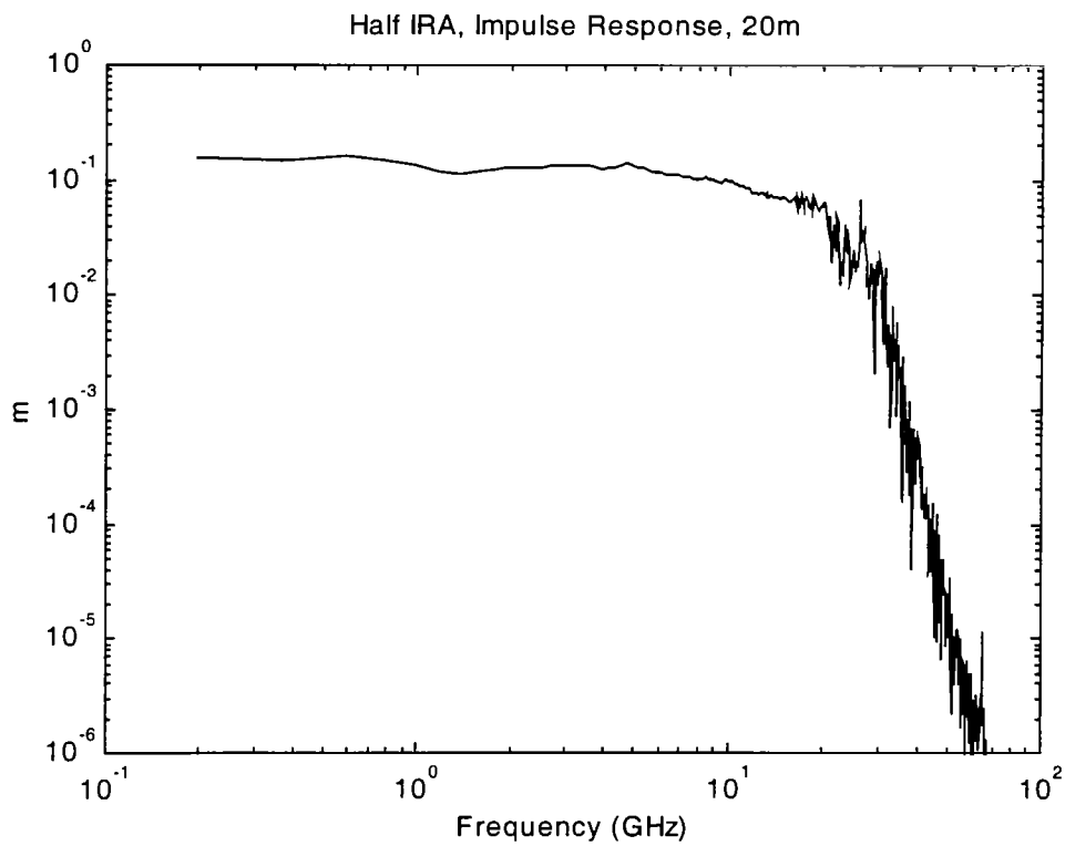
Figure 2.4 HIRA Impulse Response in Frequency Domain.
