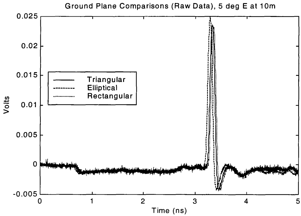
Figure 2.17. Comparison of Ground Plane Configurations.
