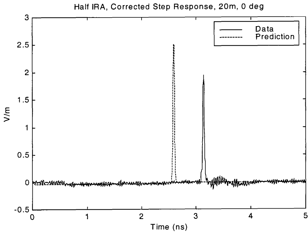
Figure 2.19. Comparison of Corrected Data and Prediction.
