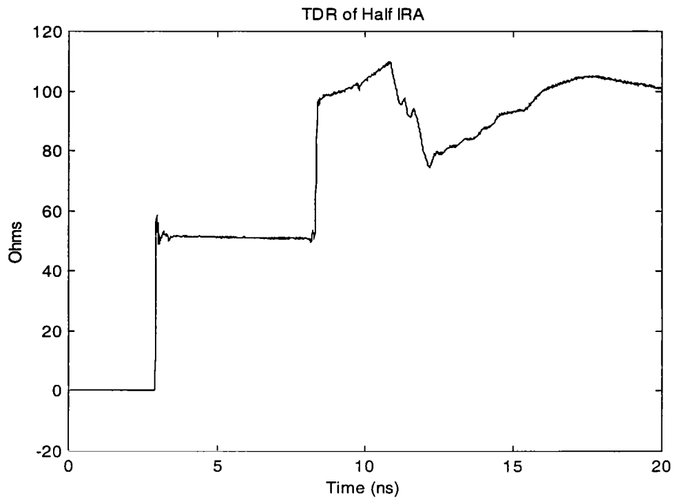
Figure 2.1 TDR of HIRA.
