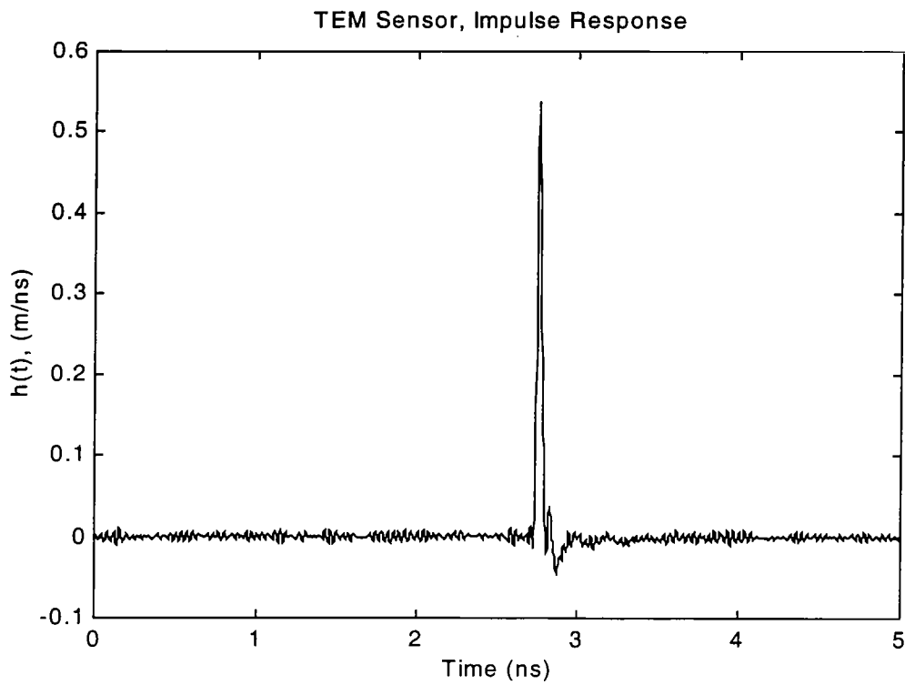
Figure 1.3. h_{\text{TEM}}(t) .
