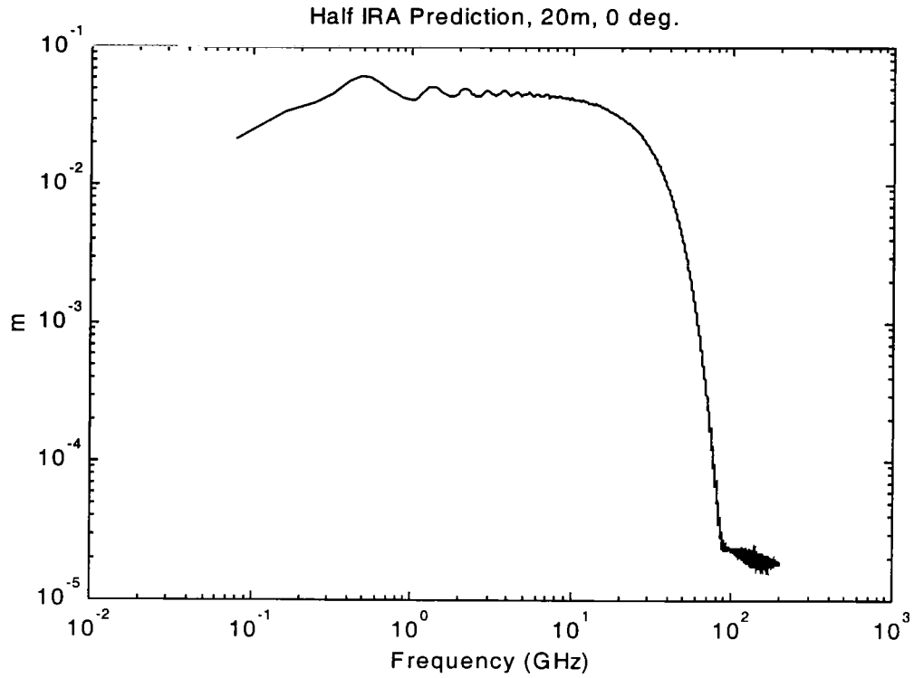
Figure 2.20. HIRA on Boresight Prediction at 20 m.
