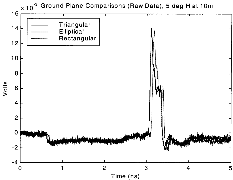
Figure 2.16. Comparison of Ground Plane Configurations.
