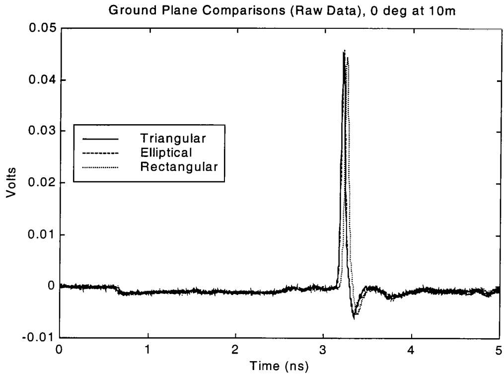
Figure 2.15. Comparison of Ground Plane Configurations.
