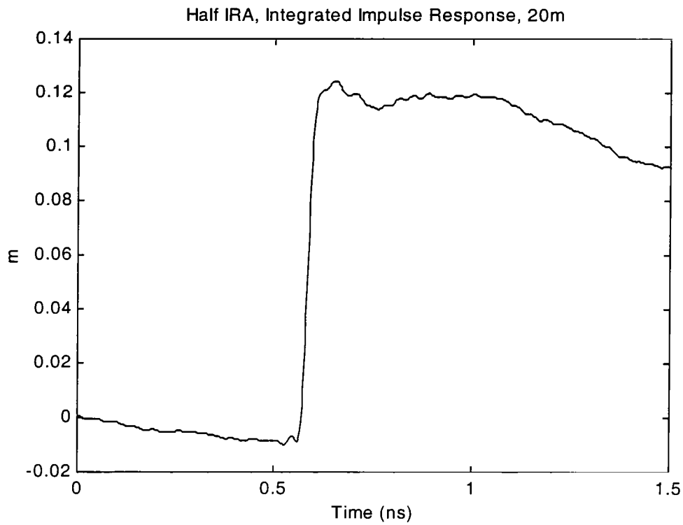
Figure 2.3 h_{\text{HIRA}}(t) dt , Effective height 0.13m.
