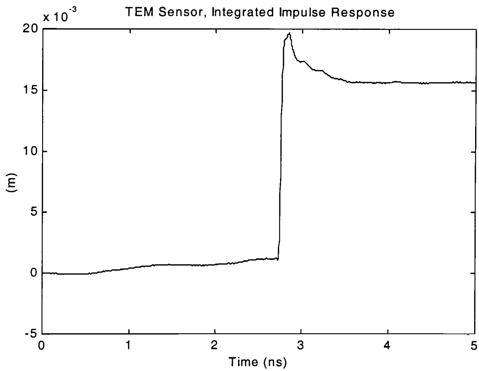
Figure 1.4. \int h_{\text{TEM}}(t) dt , Effective Height \approx 17\text{mm} .
