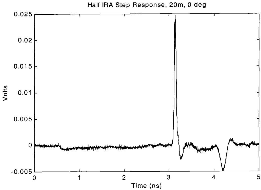
Figure 2.18. Measured Voltage on Boresight at 20 m Showing Ground Bounce.
