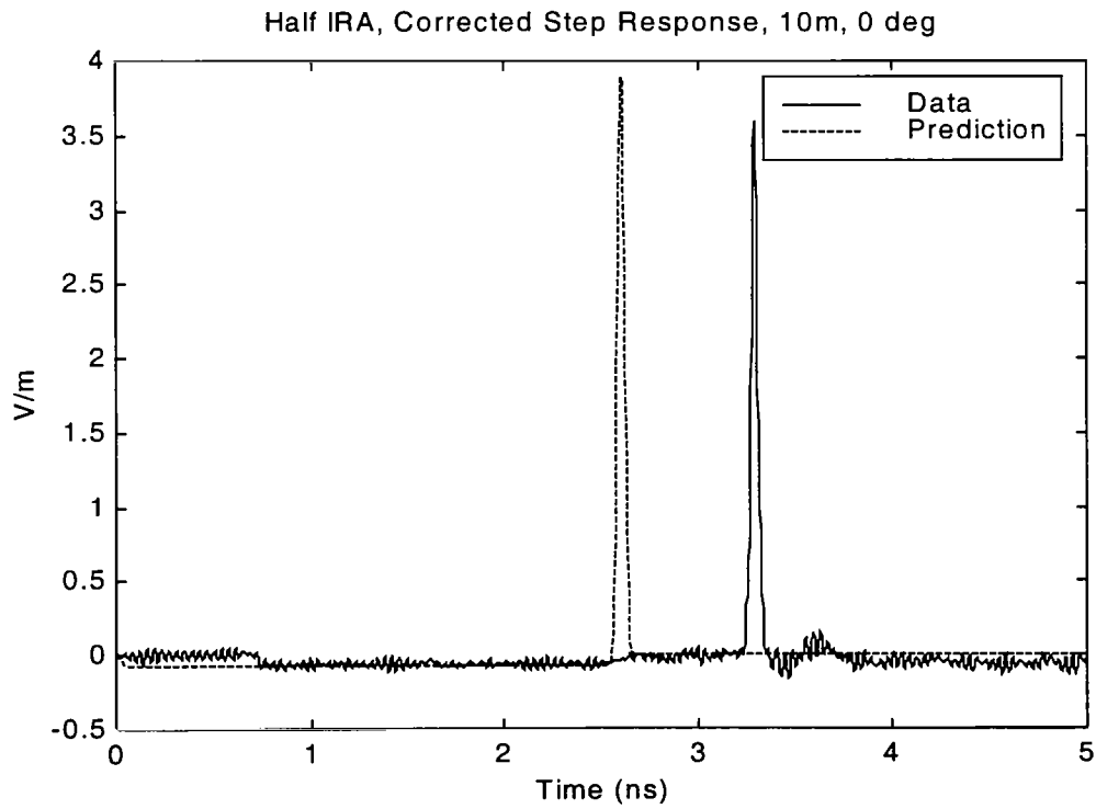
Figure 2.10. Comparison of Corrected Data and Prediction.
