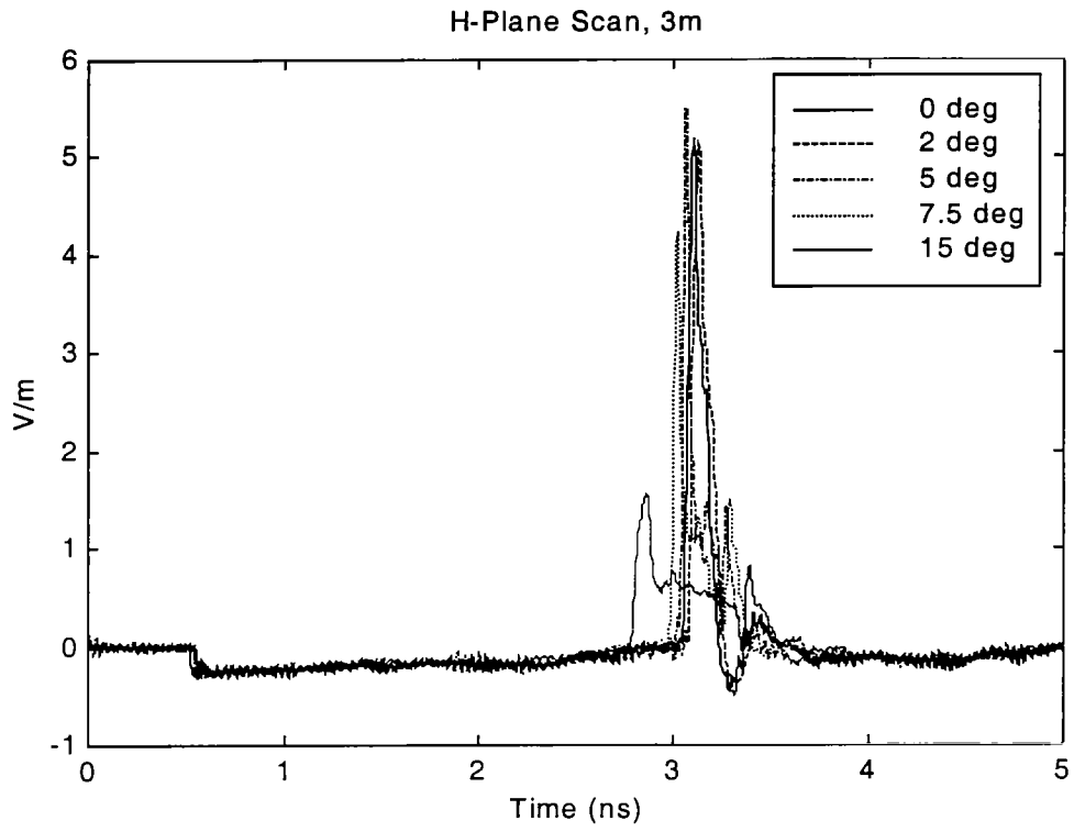
Figure 2.7. H Plane Scan at 3 m.
