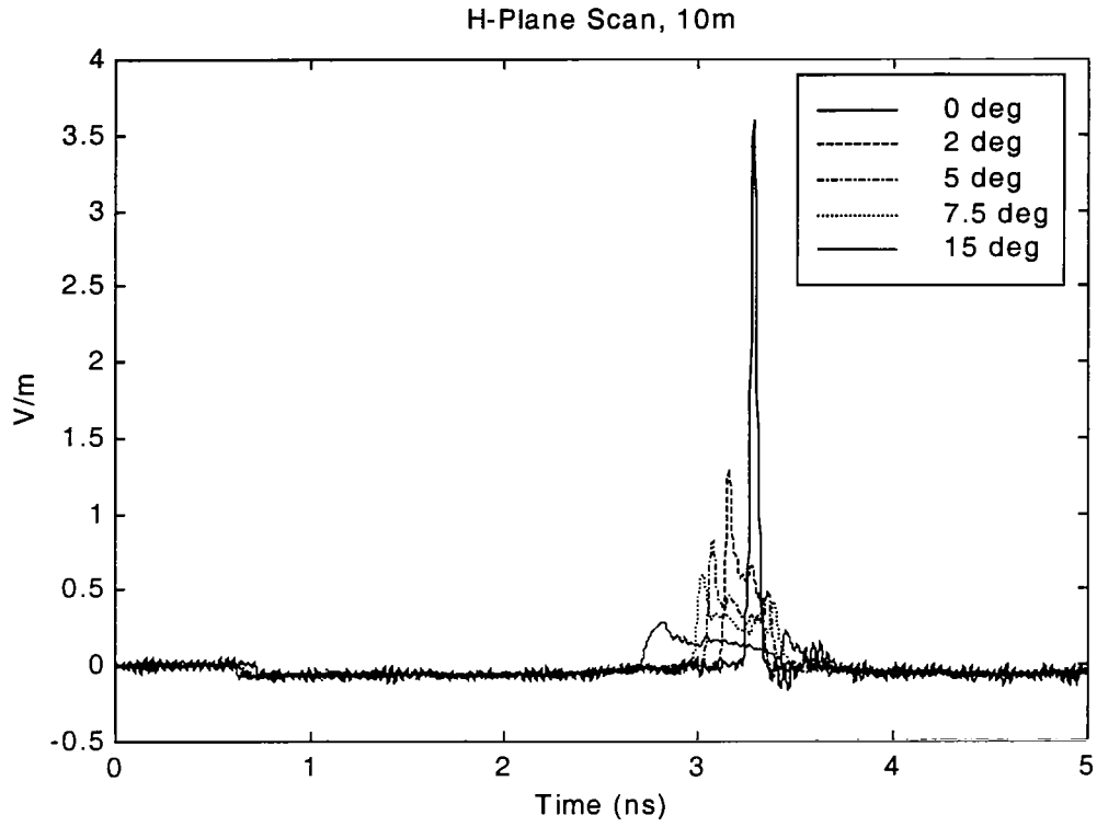
Figure 2.11. H Plane Scan (to right) at 10 m.
