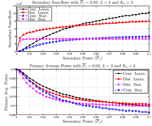
Fig. 6: Primary and Secondary Performance vs. \bar{P}_j .
