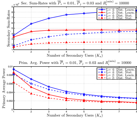
Fig. 7: Primary and Secondary Performance vs. K_s .
