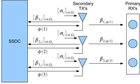
Fig. 4: Secondary System Decision Center (SSDC) Operation.
