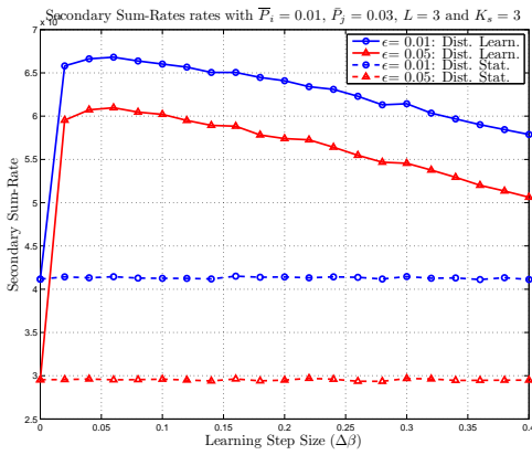
Fig. 8: Secondary Sum Rates vs. \Delta\beta .
