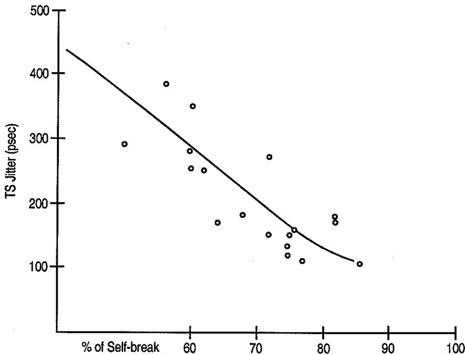
Figure 98. TS jitter vs. percent of self-break for a gap of 0.226 cm with nitrogen and mushroom stick-out 38% (from Table 11).
