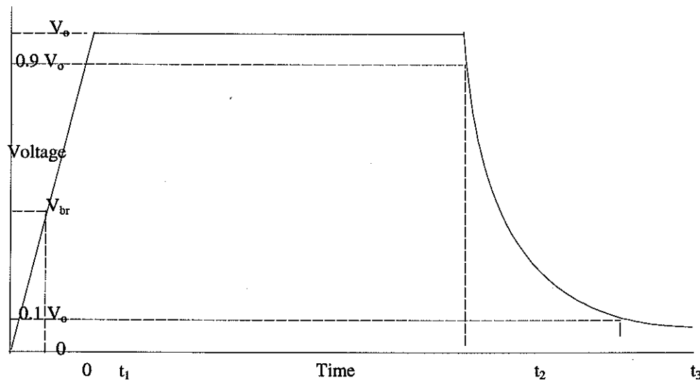
Figure 60. Breakdown delay time.
