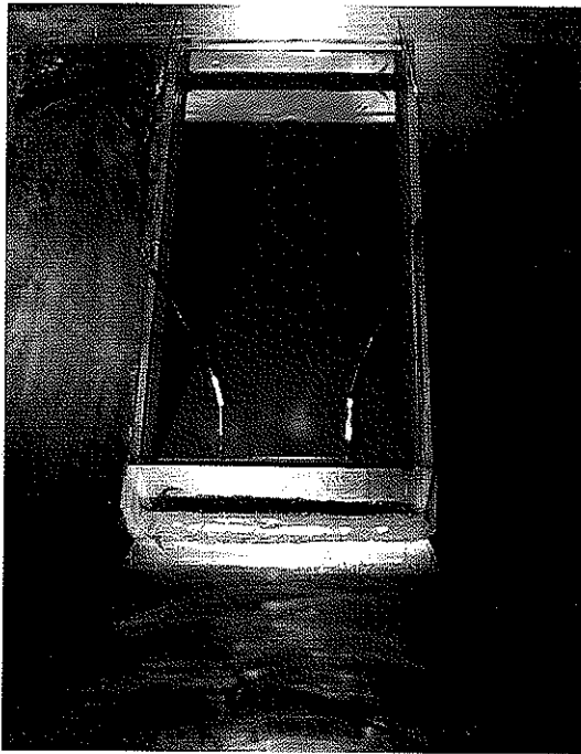
(a) TEM Horn Antenna in an oil bath
