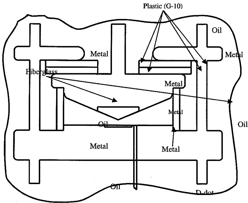
Figure 11. Monocone test fixture.
