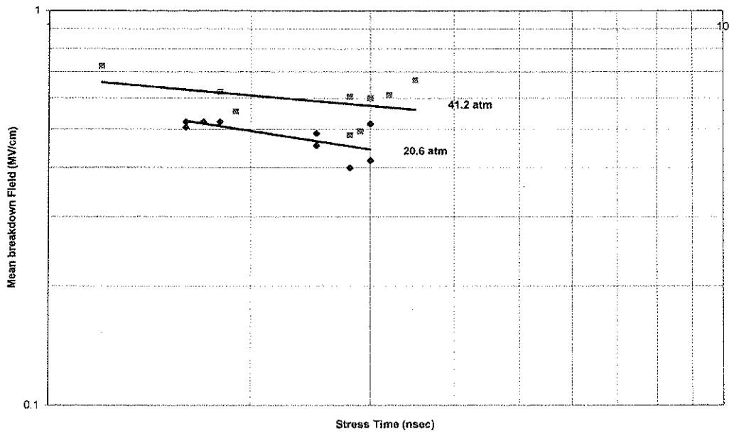
Figure 58. Point plane 30% SF6/70% air positive polarity.
