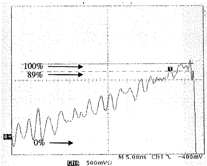
Figure 17. Typical monocone charging waveform measured by the resistive monitor.
