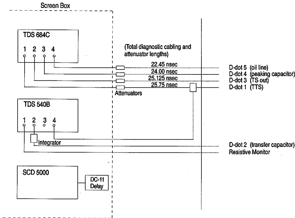
Figure 89. Trigger coax calibration pulse (integrated D-dot).
