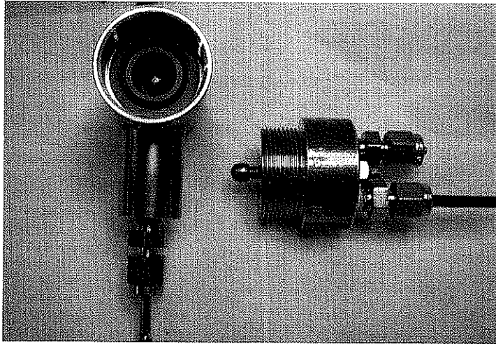
Figure 74. Self-breaking trigger switch.
