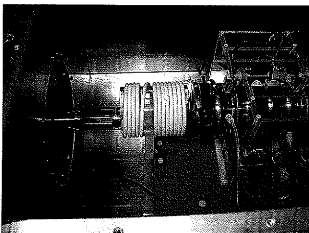
Figure 18. Marx with added series inductor.
