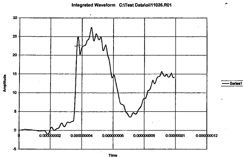
Figure 111. Output voltage from integrated oil line D-dot output voltage ~280 kV.
