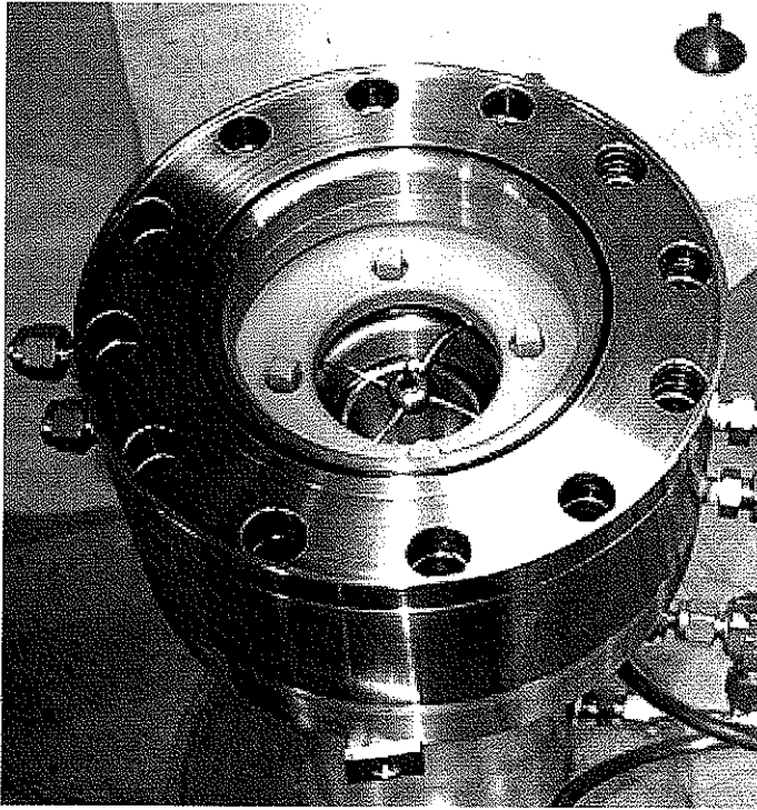
Figure 80. UV illuminator downstream electrode with Torlon support for peaking capacitor.
