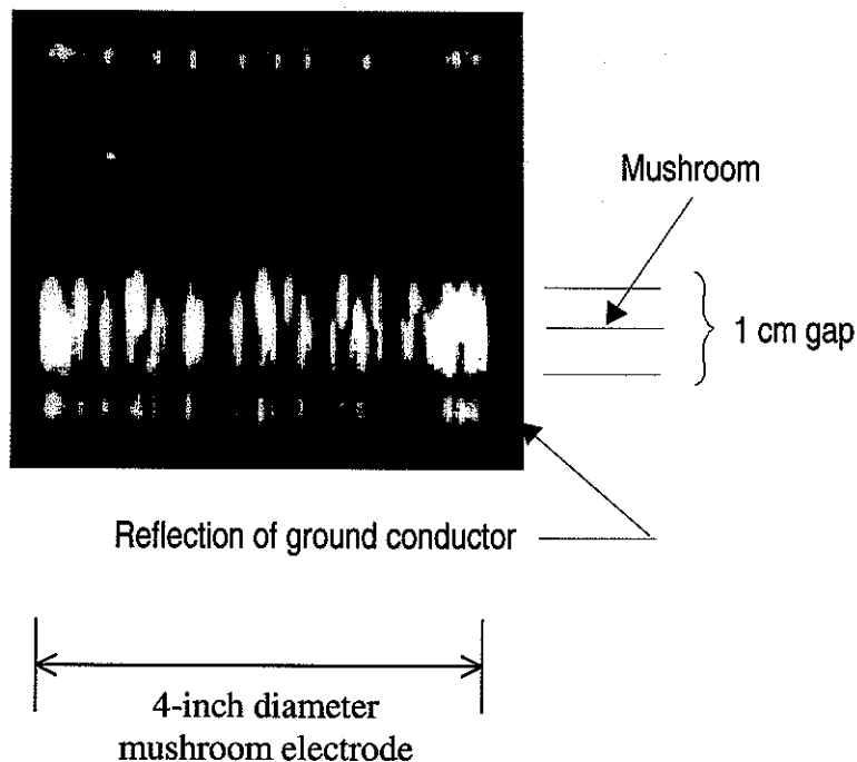
Figure 6. Channeling photo of Aesop demonstration switch.
