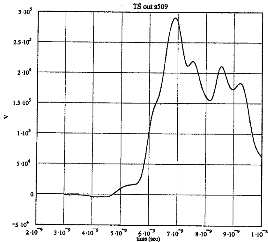
Figure 86. Transfer switch output waveform (integrated D-dot).
