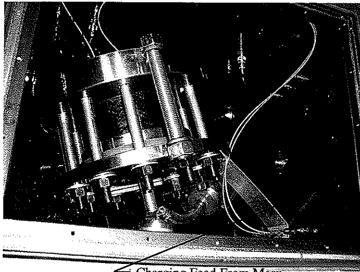
Figure 12. View of monocone test fixture in oil tank.
