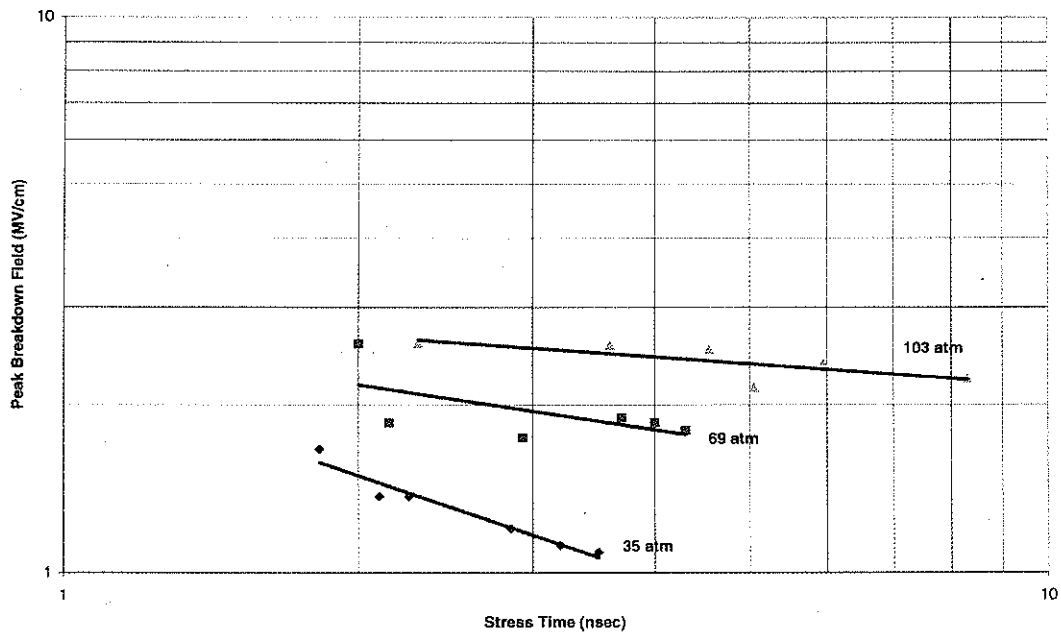
Figure 24. Monocone nitrogen negative polarity
