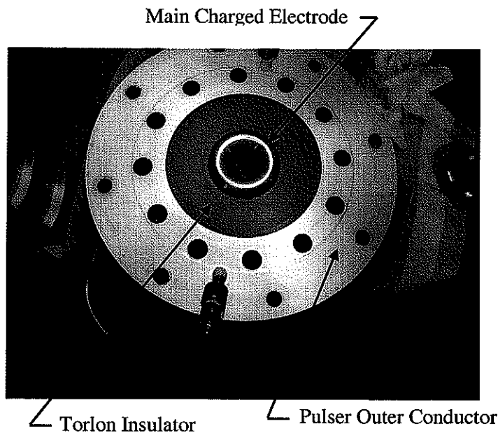
Figure 77. Transfer switch charged electrode with mushroom removed.
