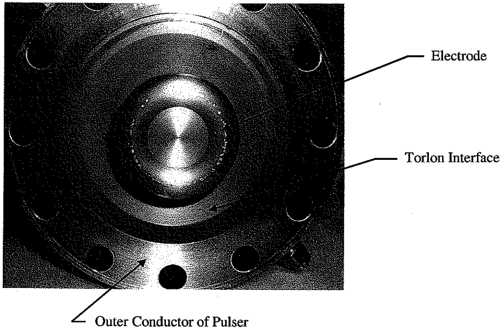
Figure 78. Transfer switch downstream electrode.
