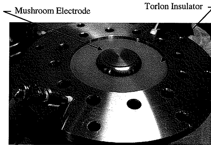
Figure 76. Transfer switch mushroom electrode.
