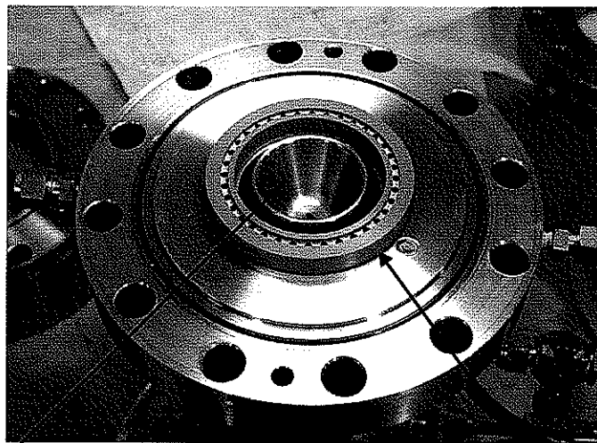
↙ Downstream Output Switch Electrode Torlon Peaking Capacitor Body ↘
