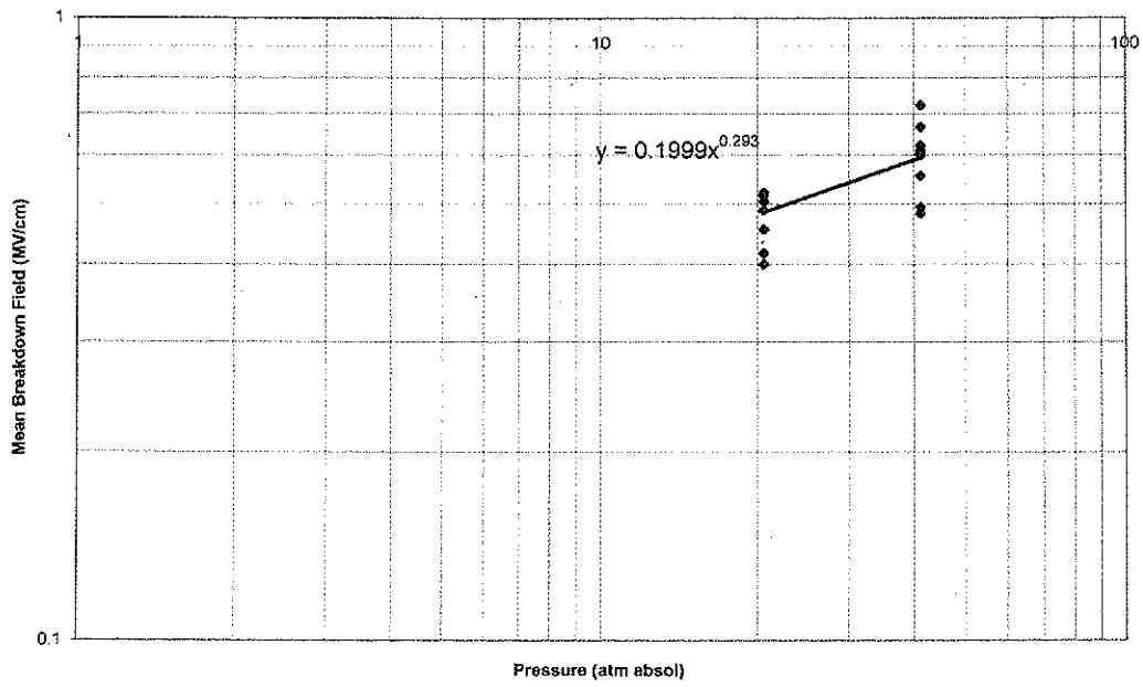
Figure 57. Point plane 30% SF6/70% air positive polarity.
