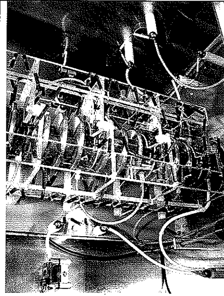
Figure 66. Marx generator.
